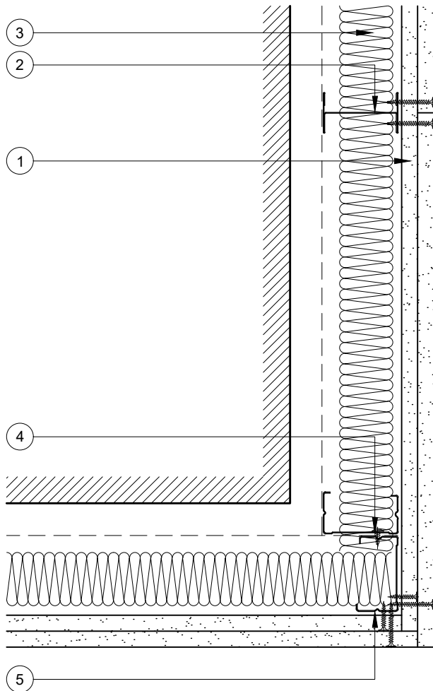
External Corner
