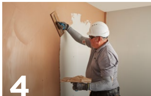
4 Thistle plaster is applied with firm pressure, built out to the required thickness in two applications and trowelled to a smooth matt finish. When applying ThistlePro FastSet Finish, a single mix for both first and second coat is recommended.
