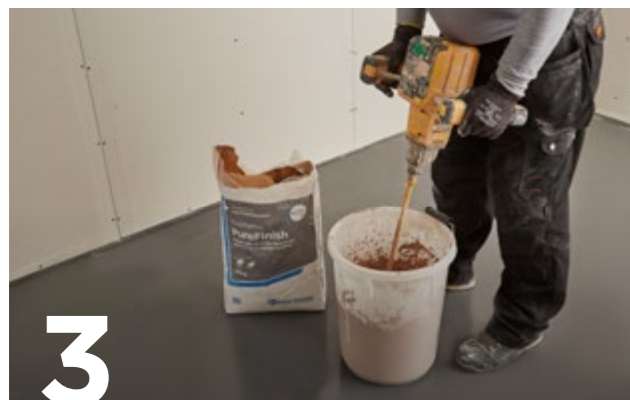
3 Thistle plasters should be mixed by adding to clean water and using clean mixing equipment. Contamination from previous mixes must be avoided as this can adversely affect the setting time and strength.
