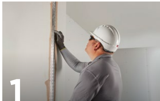
1 A Thistle Thin Coat Angle Bead is fixed to the plasterboard angle by embedding in dabs of finish plaster.
