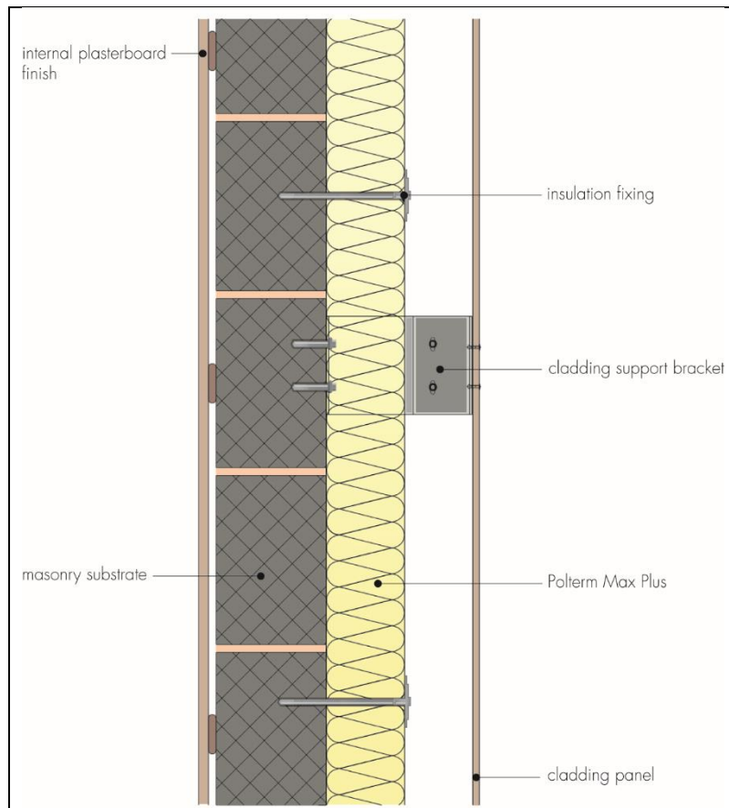
Figure 3 Masonry substrate
