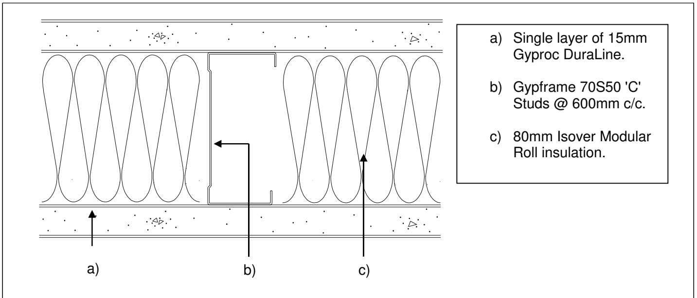
Figure 1. Horizontal cross section view
