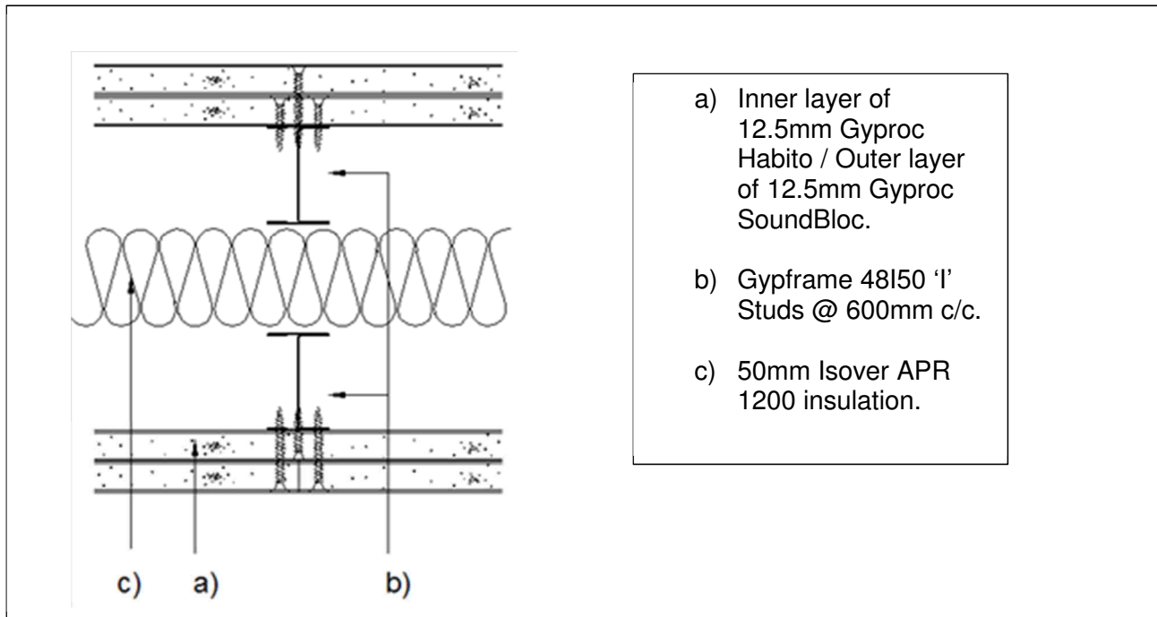
Figure 1. Horizontal cross section view
