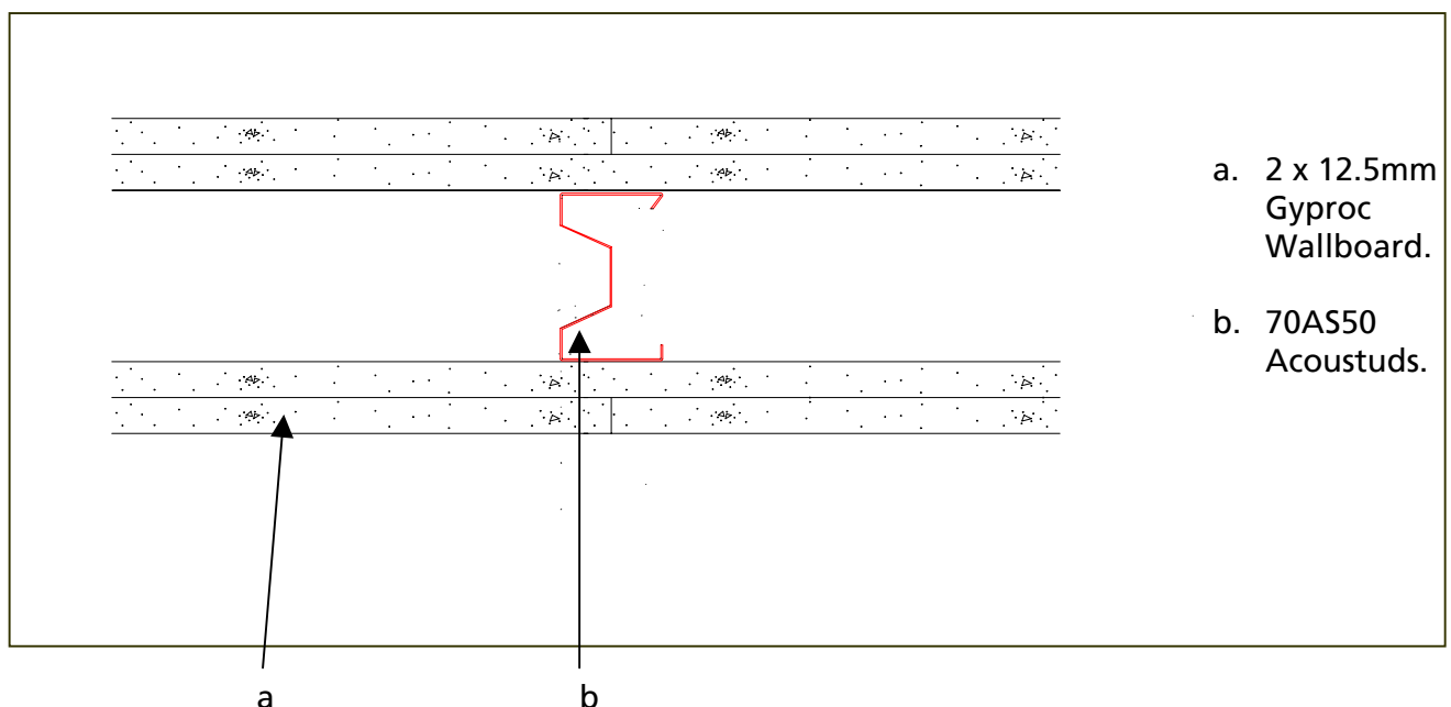
Figure 1. Cross-section through the partition.
