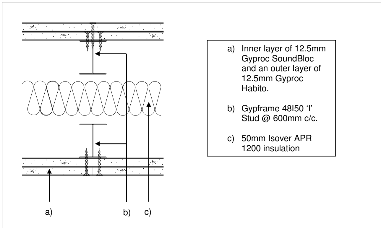
Figure 1. Horizontal cross section view
