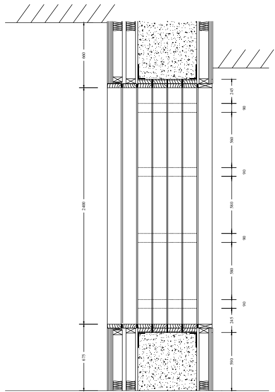
Cross section of test aperture
