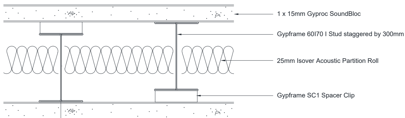
Figure 1. Horizontal cross section – Gypwall staggered metal stud partition with 60 mm Gypframe I stud framework clad each side with a single layer of 15 mm Gyproc SoundBloc 15mm and 25 mm Isover APR 1200 in the cavity.
