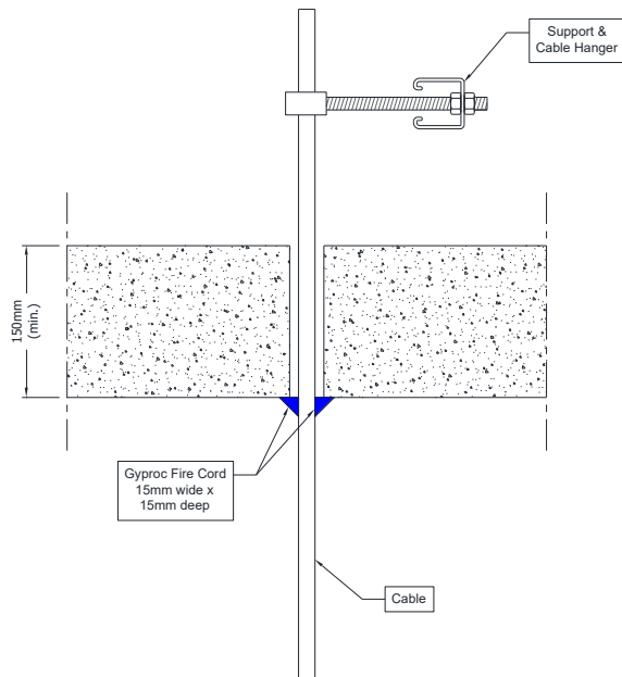
Construction details:
