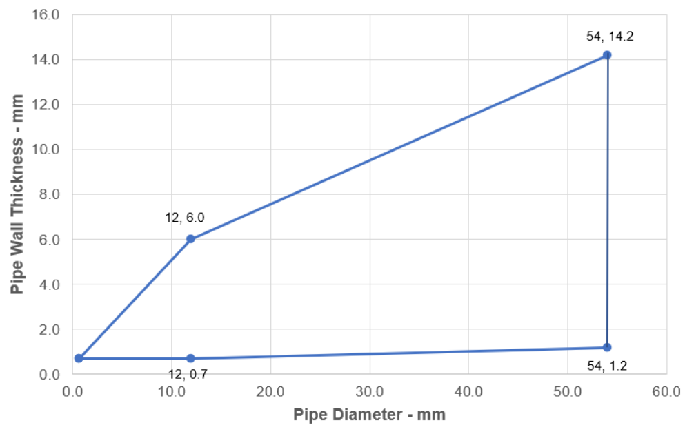
Copper or Steel Pipes with 30-80 mm Thick Insulation - EI 240, C/C
