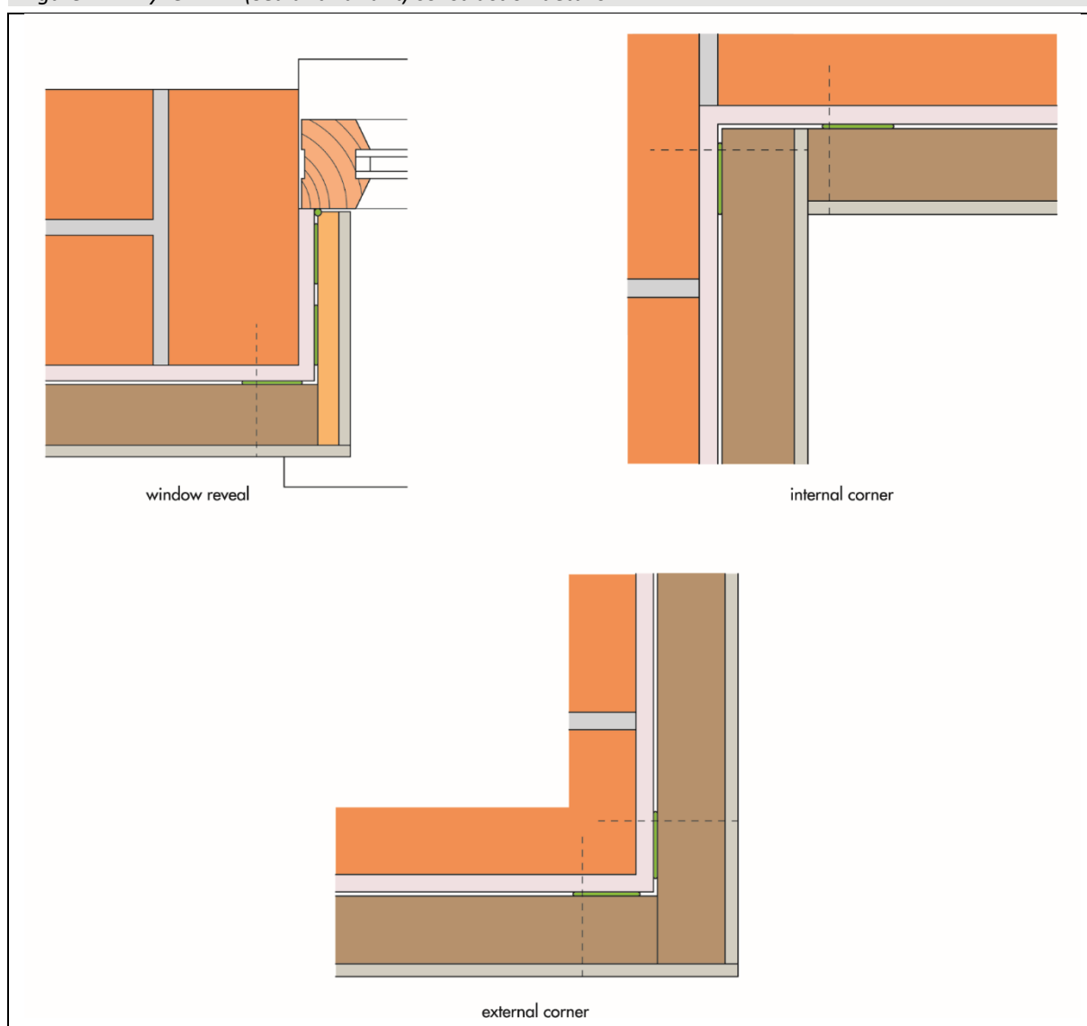
Figure 2 DriLyner DAB (Sealant Variant) construction details
